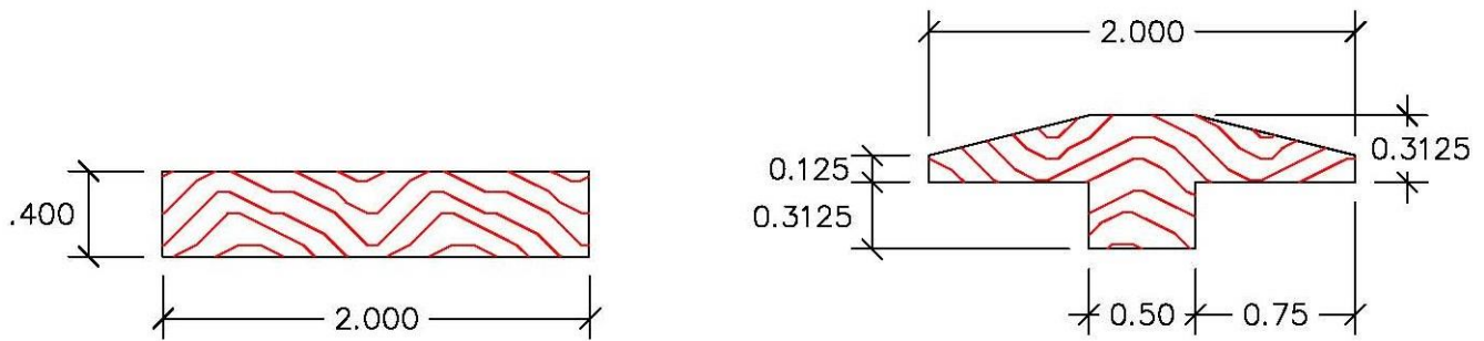
Type "C" Flat Strip
