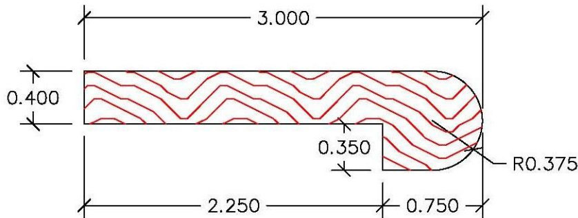
Flush Stair Nosing
