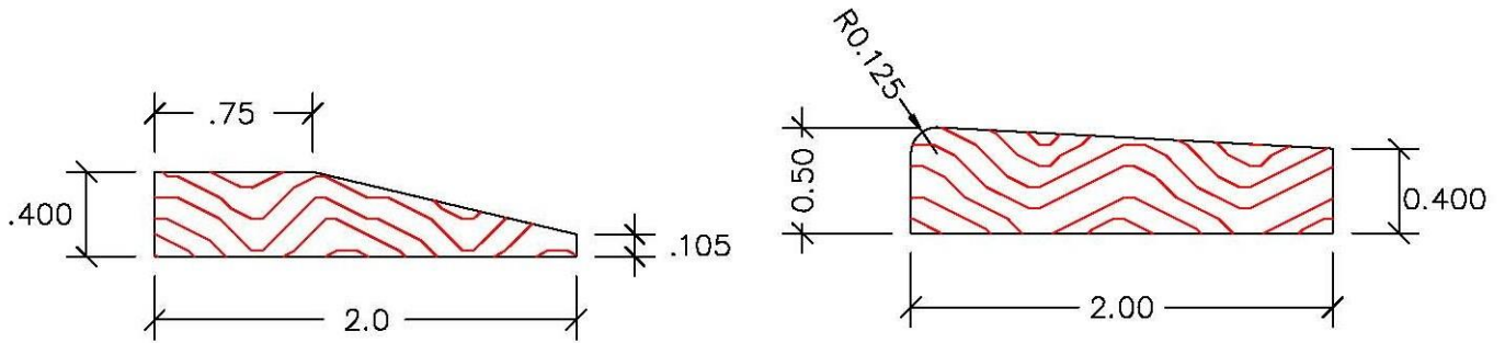
Type "A" Flush Reducer
