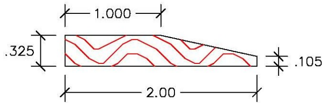
Type "A" Flush Reducer
