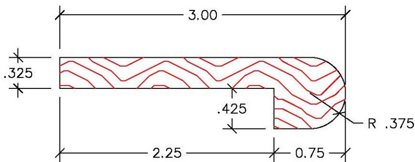
Flush Stair Nosing
