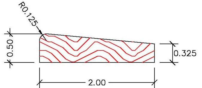
Type "B" Bi-Level Reducer
