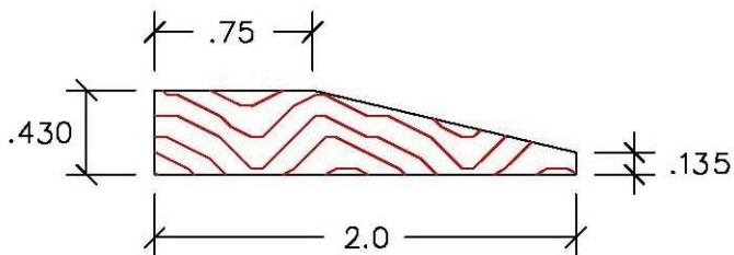
Type "A" Flush Reducer
