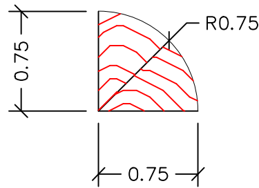
4" Square Wall Base (Effective 2/1/16) 3/4" Quarter Round
